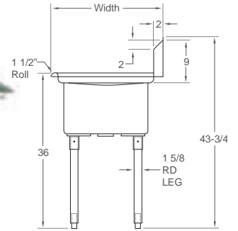
PROFILE DRAWING
